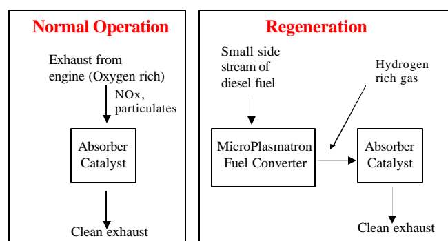
Figure 2. Diesel engine emissions aftertreatment concept
